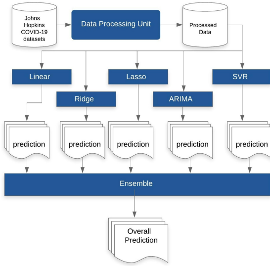
Figure 2: Ensemble model for prediction
