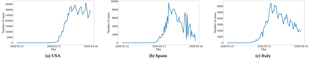
Figure 1: Cases per day for USA, Spain and Italy - the three countries with the maximum number of confirmed cases
